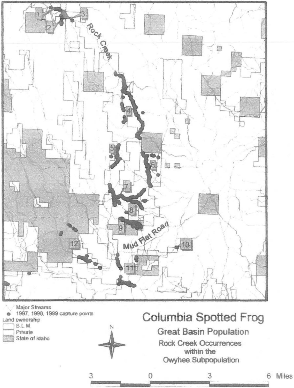
Figure 1. Rock Creek study area within the Owyhee subpopulation. Numbers represent the twelve element occurrences surveyed.
