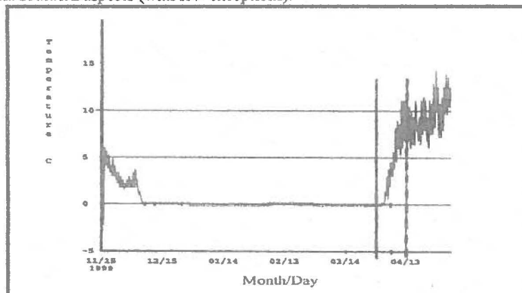
Figure 5. Temperature record for the oviposition site at Sam Noble pond #1a. Solid red line represents April 1, dotted red line represents the beginning of amplexus, and oviposition was from April 16-21.
