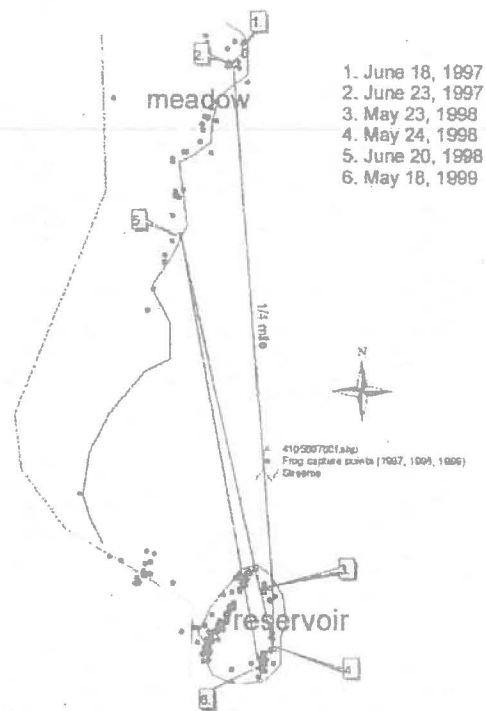
Figure 8. Migrational movement over a three-year period of one male between summer foraging and winter hibernation sites. (Black line follows capture locations chronologically, although movement probably occurred along the wet corridor to the west.)
