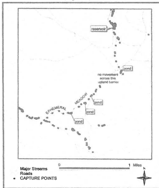
Figure 3. Spotted frogs were not captured in adjacent drainages. The most promising location would have been this 0.25 mi distance between two occurrences.
