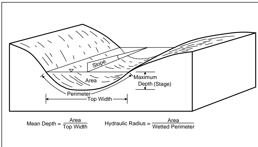
Figure 6. Definition diagram for hydraulic parameters.
