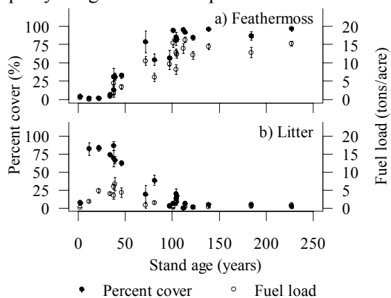
Figure 2-A. Percent cover and loading of forest floor fuels, feathermoss (a) and litter (b) relative to stand age. Error bars represent \pm one standard error.
