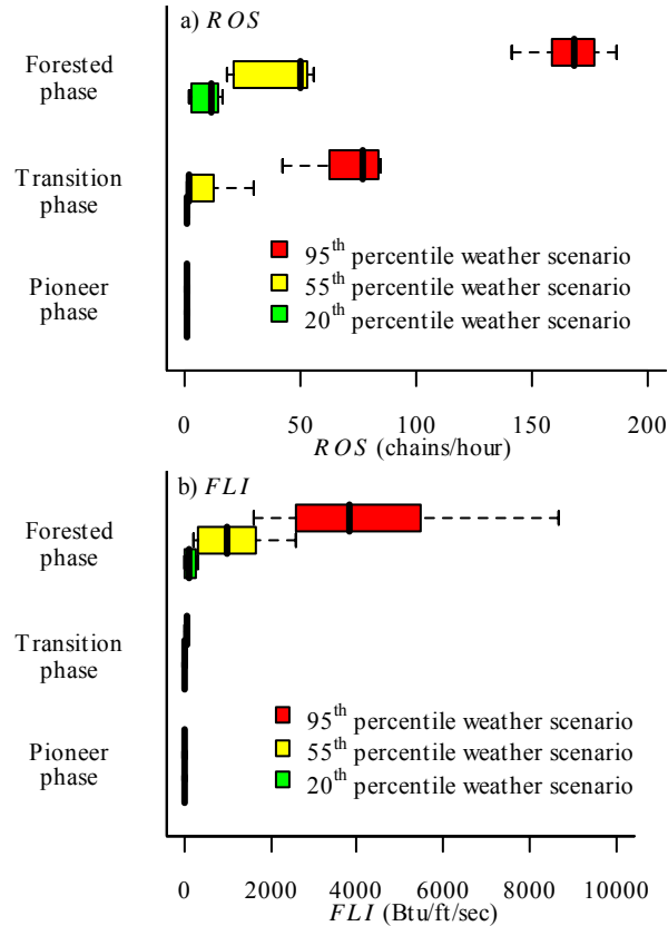
Figure 6. Predicted ROS (a) and FLI (b) relative to fuel succession phase and weather. The heavy line represents the median, the boxed area represents the first and third quartiles, and the whiskers represent minimum and maximum non-outlier values.
