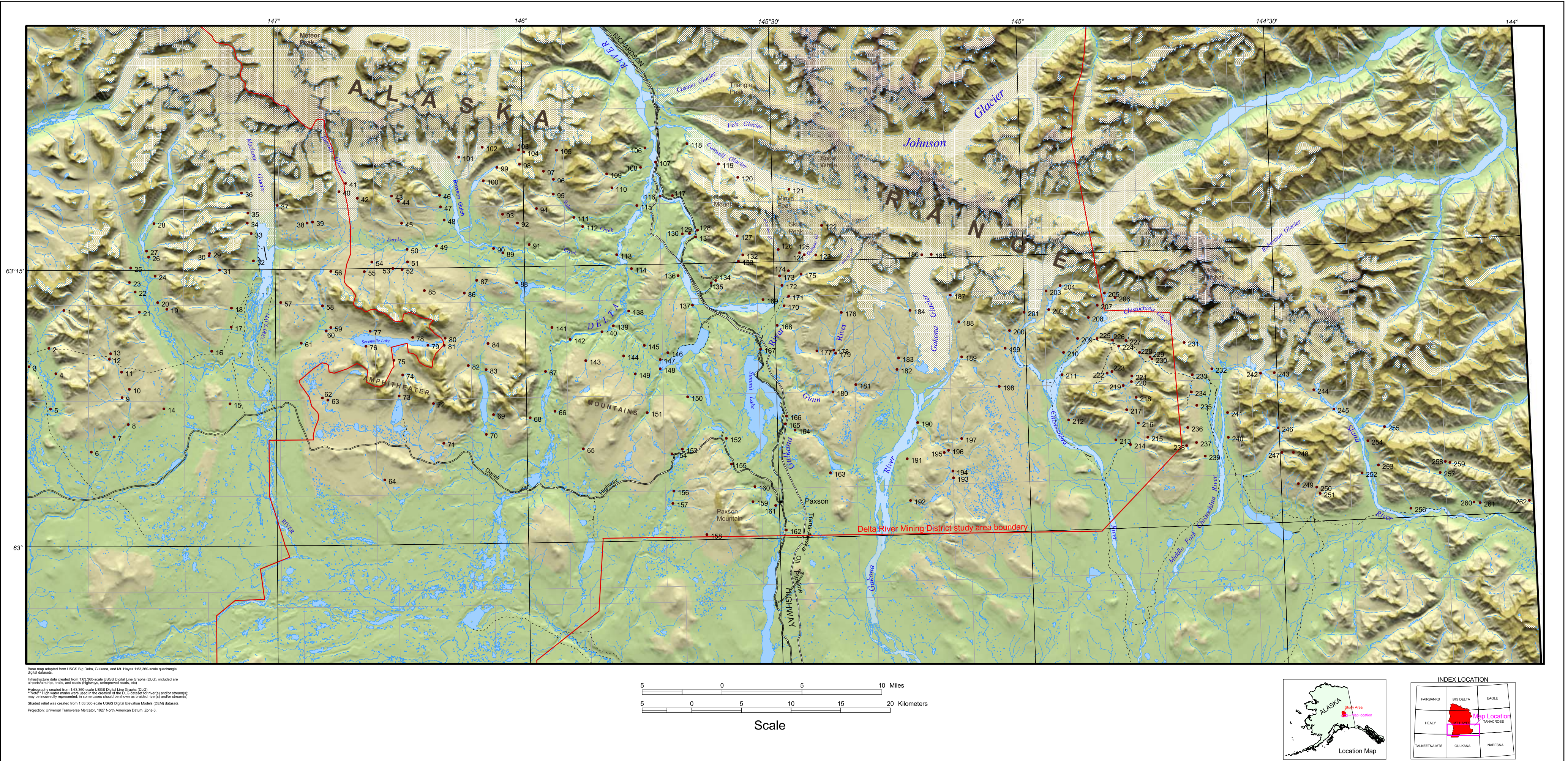
Plate 2. USGS stream sediment sample locations in the southern Mt. Hayes quadrangle, East-central Alaska (for analytical results see Appendix Table B-7).
