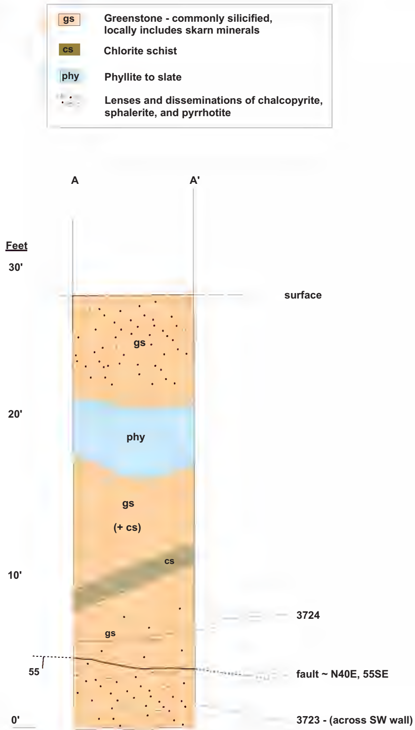
Figure 10. Cross section of the southeast face of the Northern Copper shaft. Section A A' location shown on figure 8.
