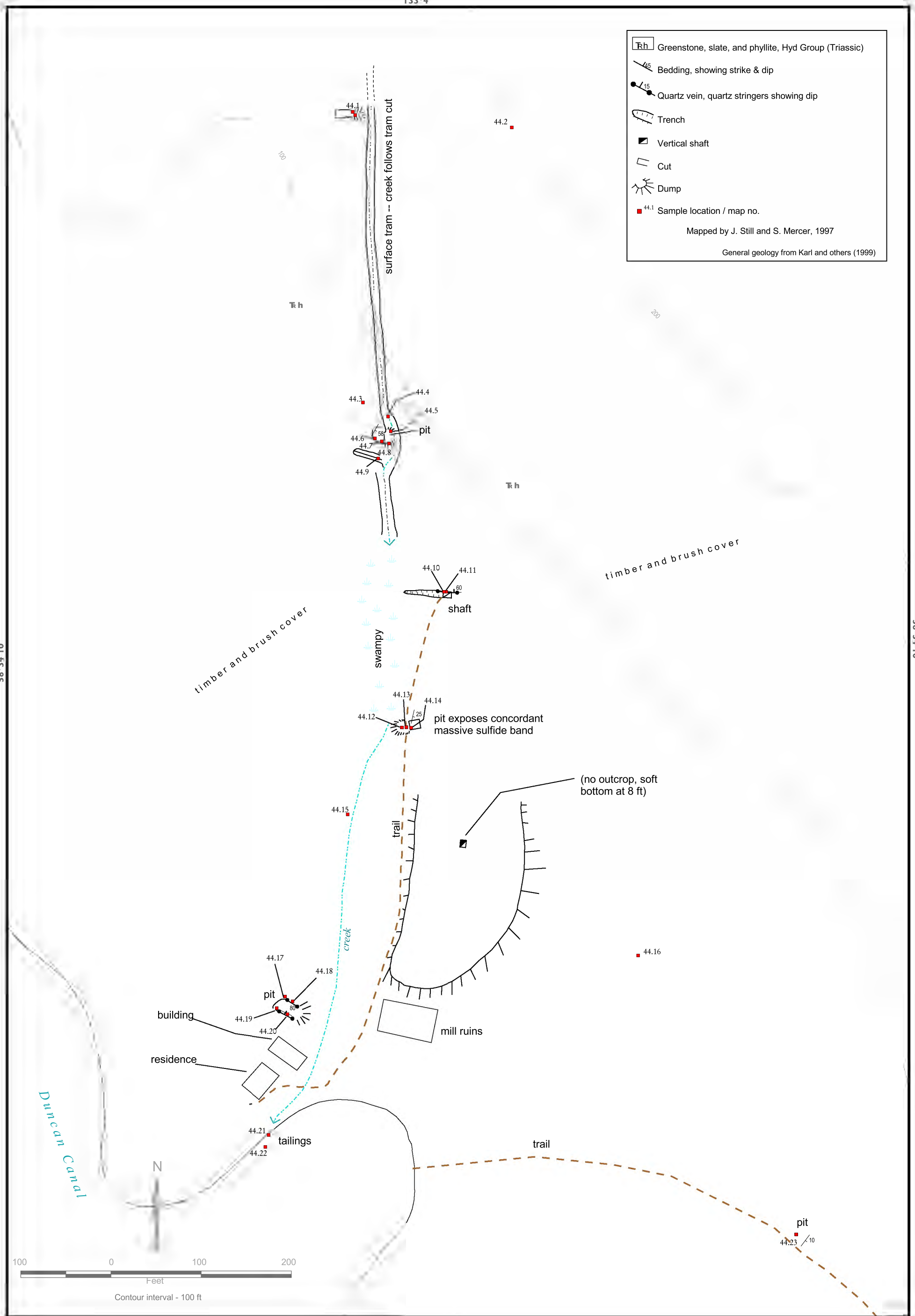
Figure 15. Map of the Helen S Mine.
