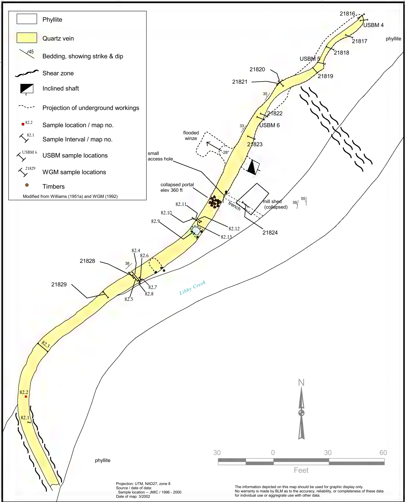
Figure 25. Map of the K & D prospect.
