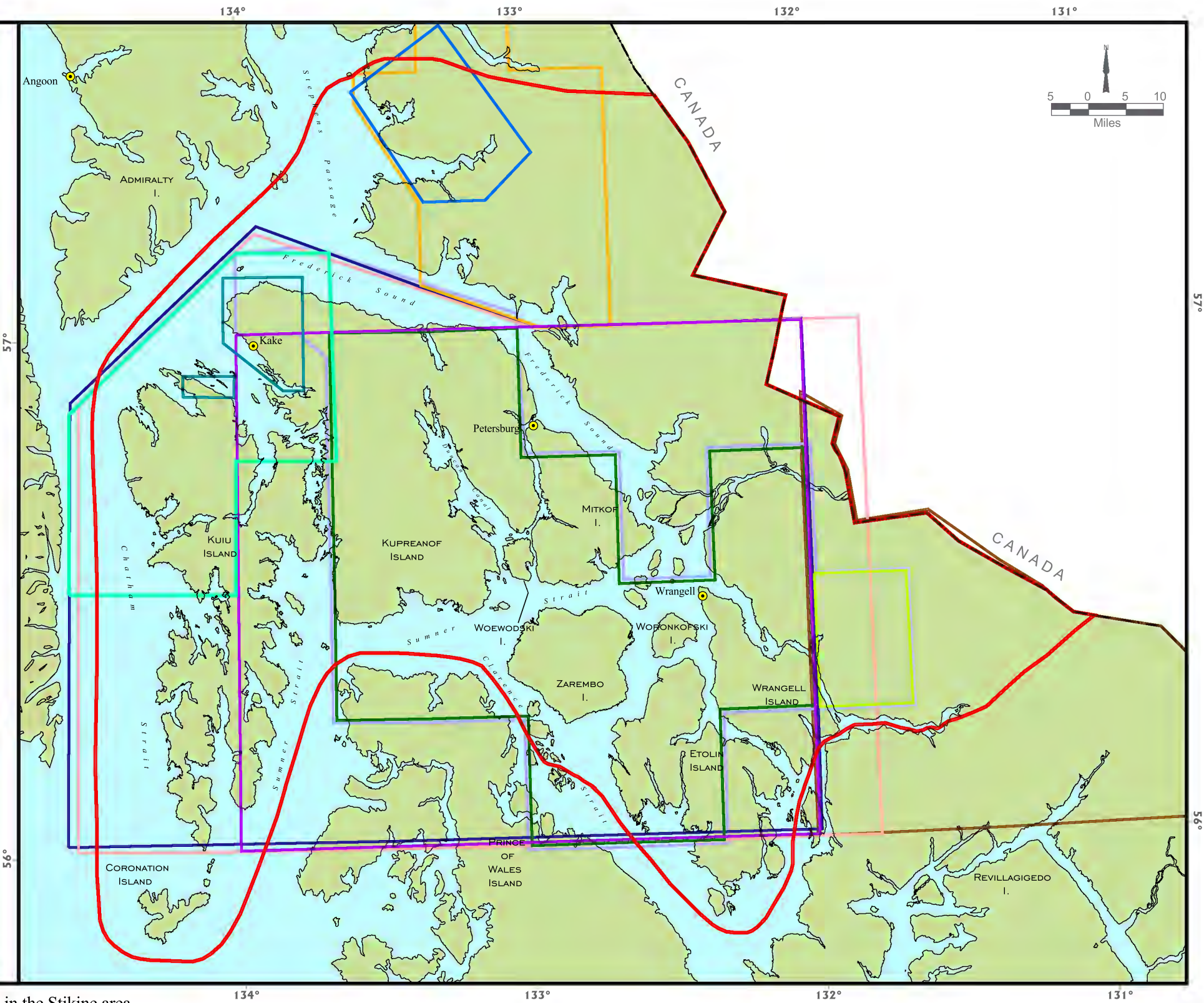
Figure 3. Map showing previous studies in the Stikine area.
