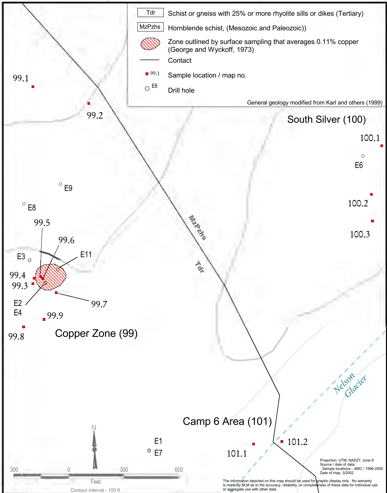
Figure 28. Map of the Copper Zone, South Silver, and Camp 6 Area prospects.
