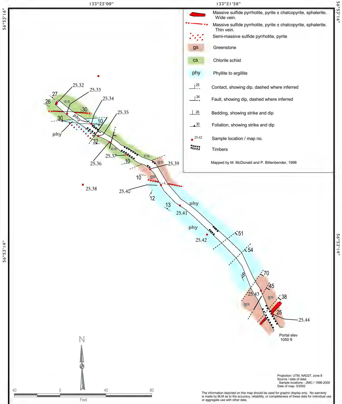
Figure 11. Map of the Northern Copper lower adit. Profile of southwest rib shown in figure 12.
