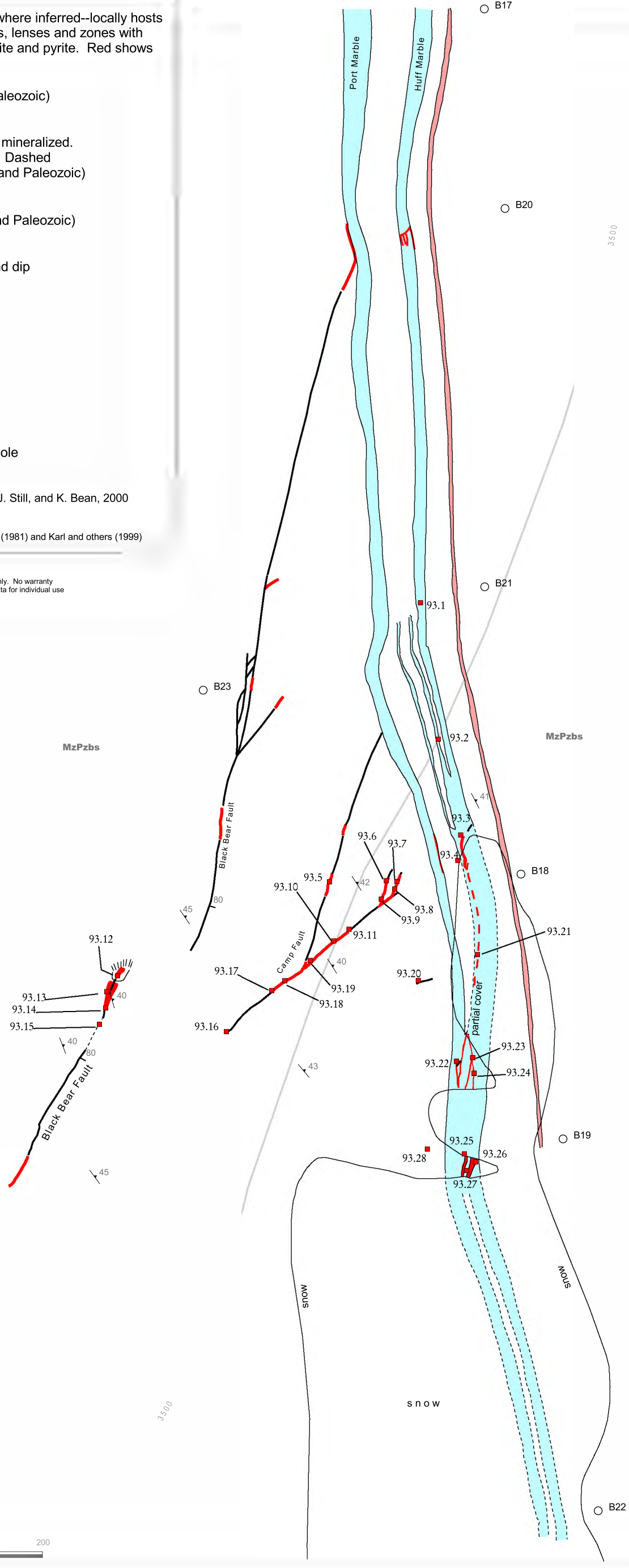
Figure 27. Map of the North Silver North prospect.
