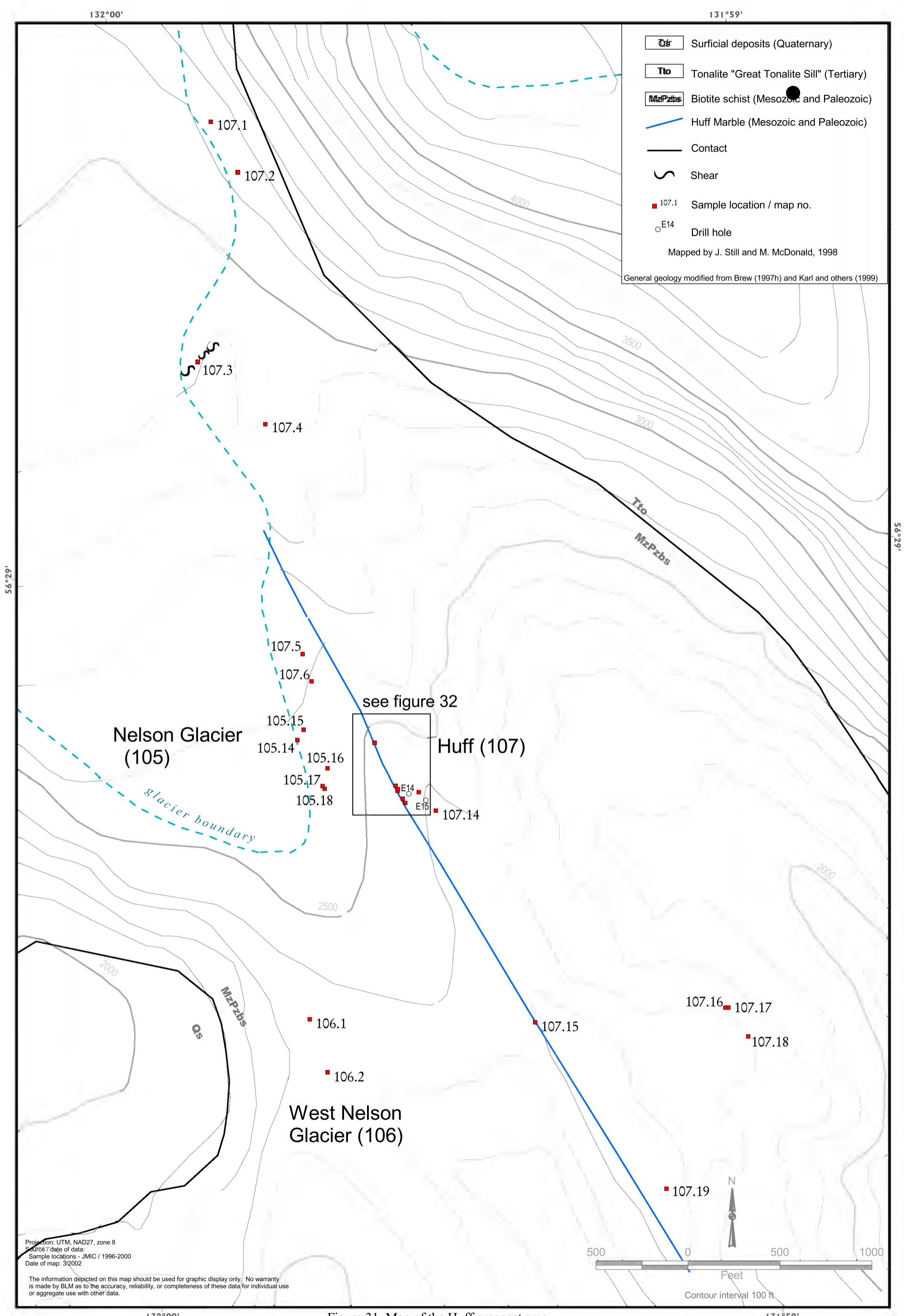
Figure 31. Map of the Huff prospect area.
