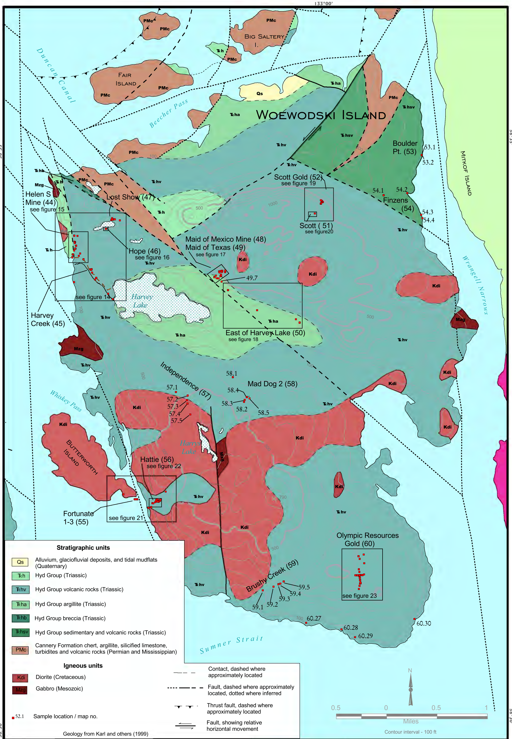
Figure 13. Map of Woewodski Island, showing prospects and geology.
