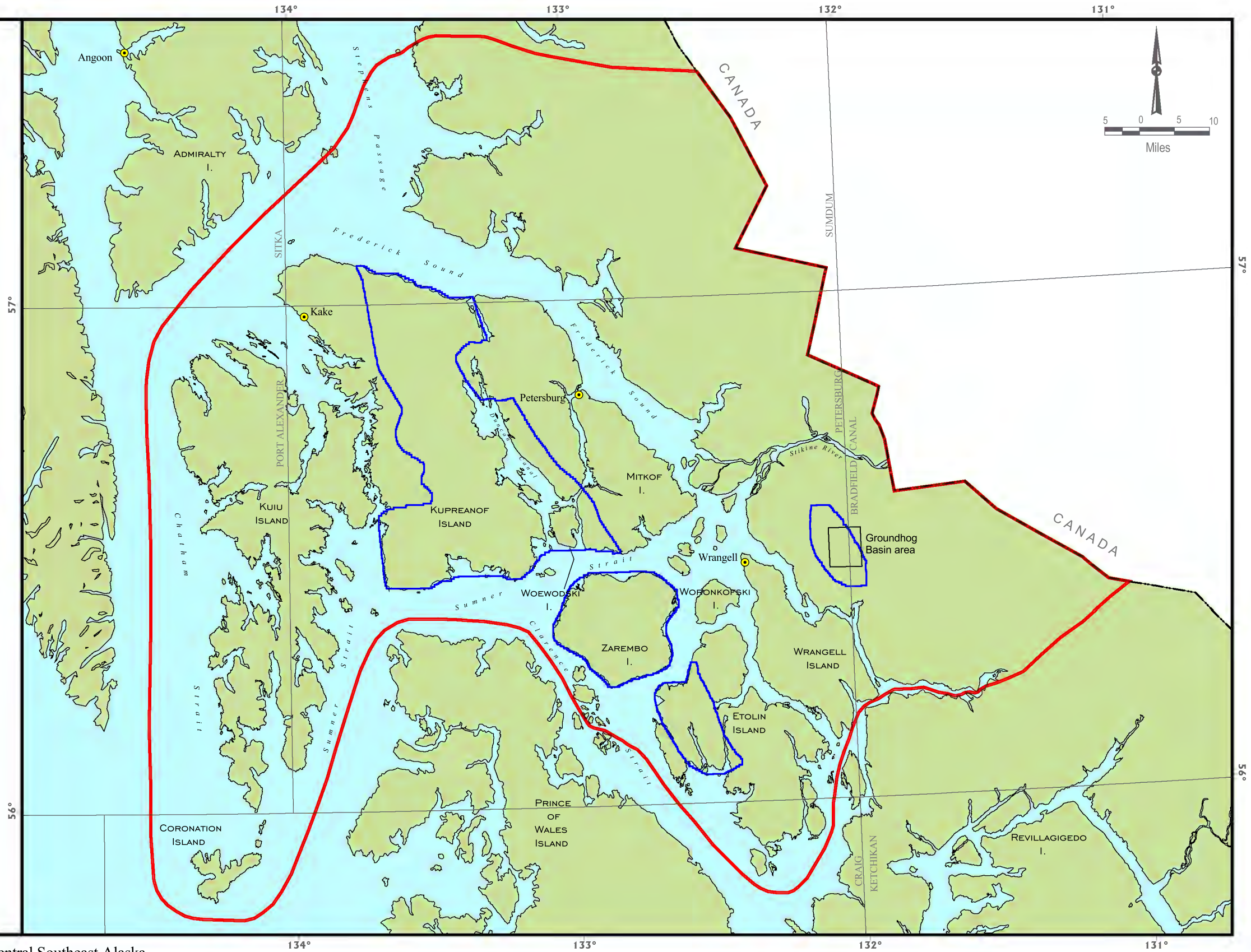
Figure 1. Location map of the Stikine area, central Southeast Alaska.
