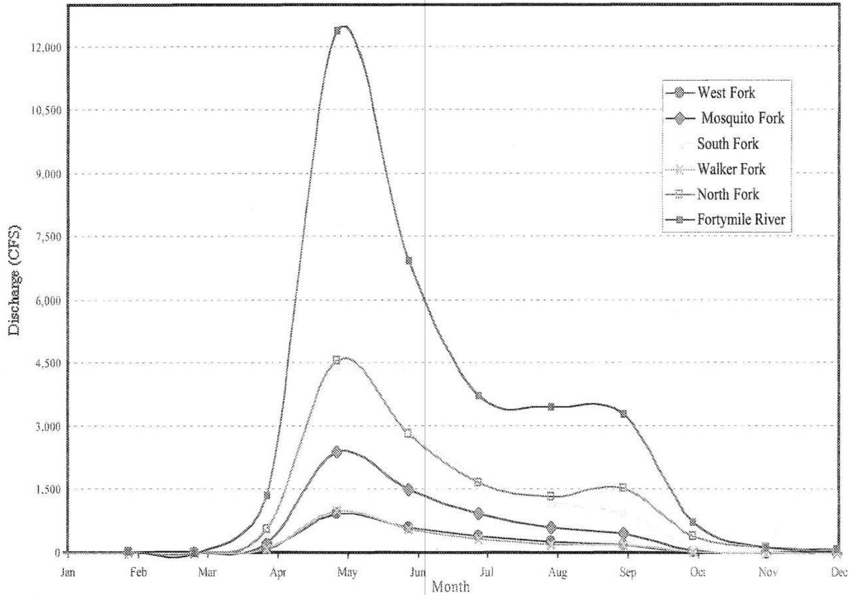
Figure 11. Monthly mean discharge hydrograph for the Fortymile River basin.
