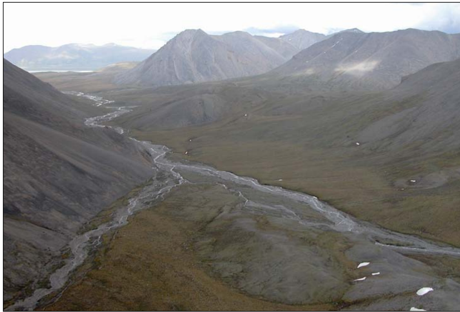
Figure 14. View to the northeast from the southwestern border of the Galbraith Lake ACEC, Utility Corridor Management Area, Alaska. Galbraith Lake is visible in the background.
