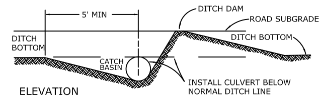
CATCH BASIN
