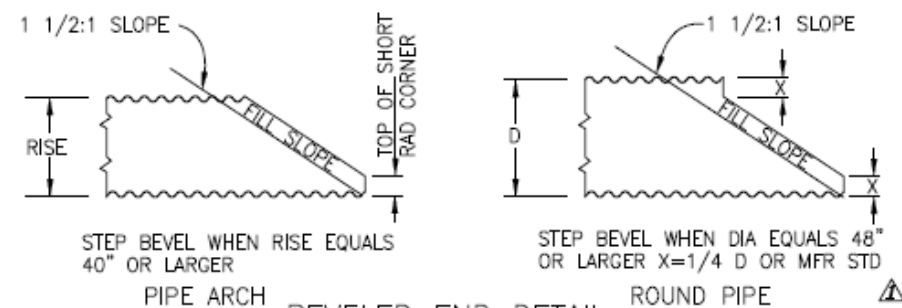
BEVELED END DETAIL
