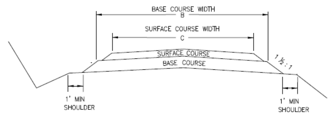
SECTION TYPE 3 CROWNED ROAD WITH ROCK
