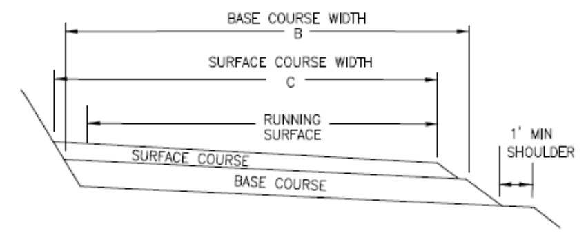
SECTION TYPE 4 – OUT SLOPE ROAD WITH ROCK
