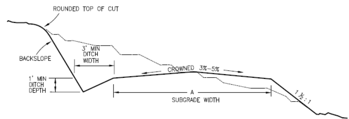
SECTION TYPE 1 – CROWNED ROAD
