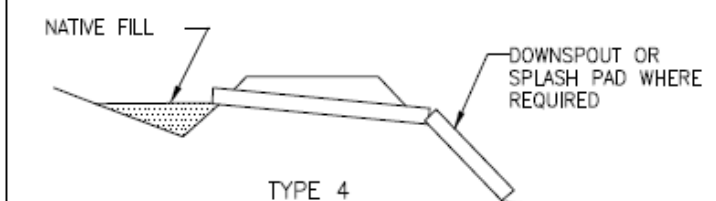
CULVERT INSTALLATION TYPES
