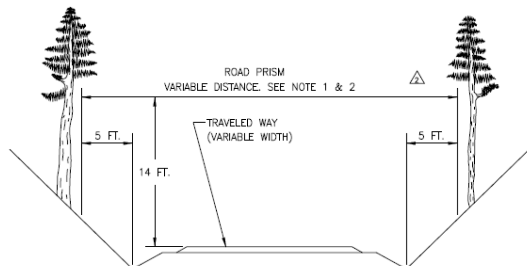
EXAMPLE 3 THRU CUT
