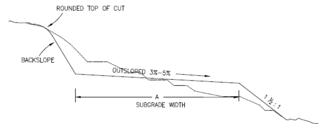
SECTION TYPE 2 – OUT SLOPE ROAD
