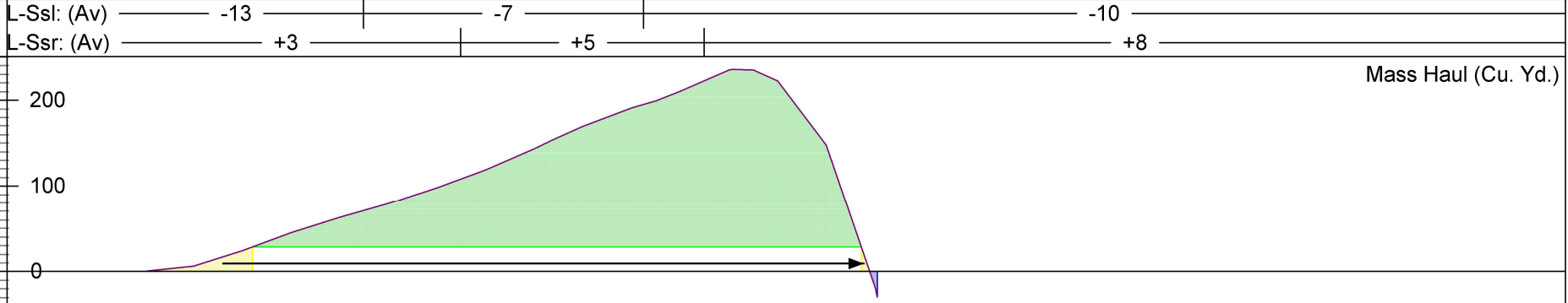
Mass Haul
