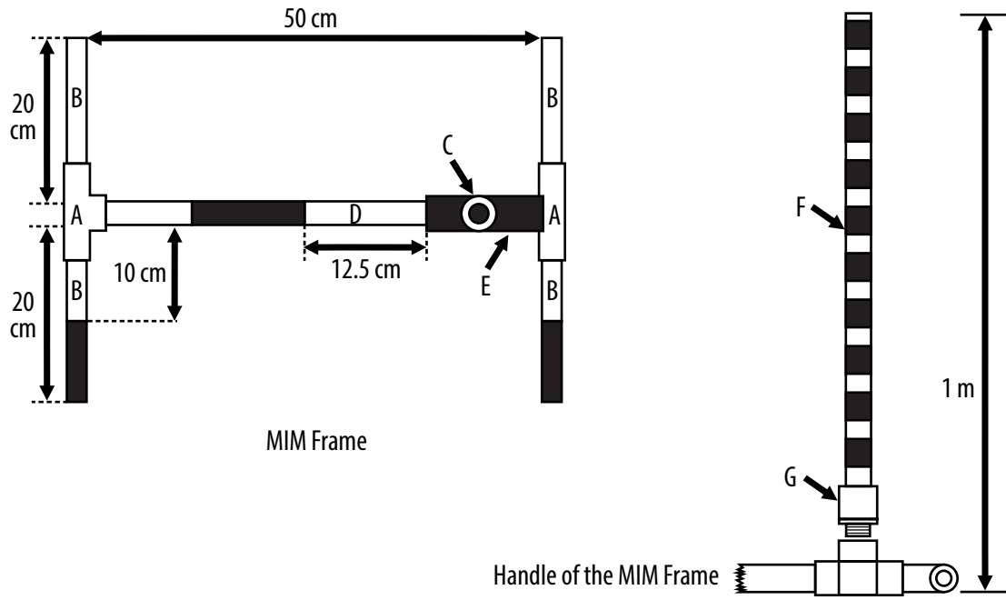
Figure R1. Schematic diagram of the MIM frame and handle.
