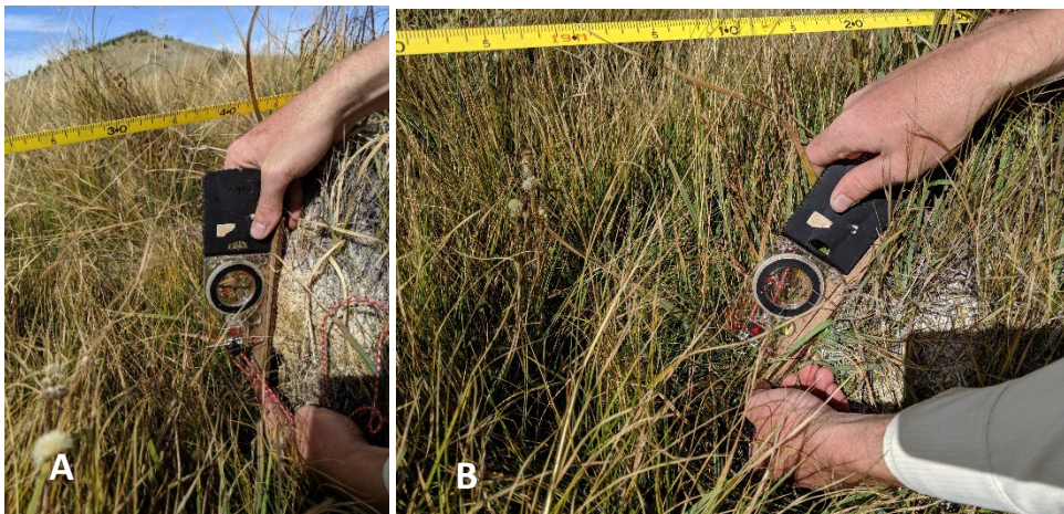
Figure 41. Measuring slope of the leading edge with a ruler and compass, showing (A) a steeper side slope and (B) a moderately shallow side slope.
