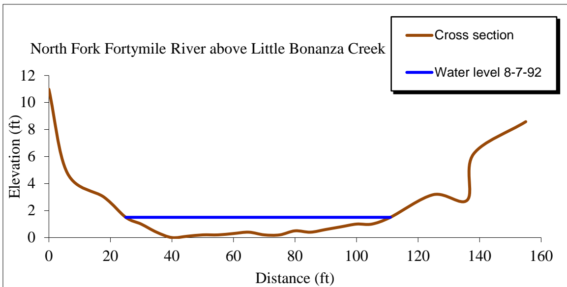
Fig. 29 The surveyed cross section on North Fork Fortymile River above Little Bonanza Creek
