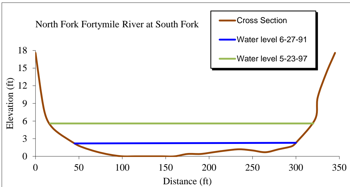
Fig. 16 Channel cross section at North Fork Fortymile River at South Fork
