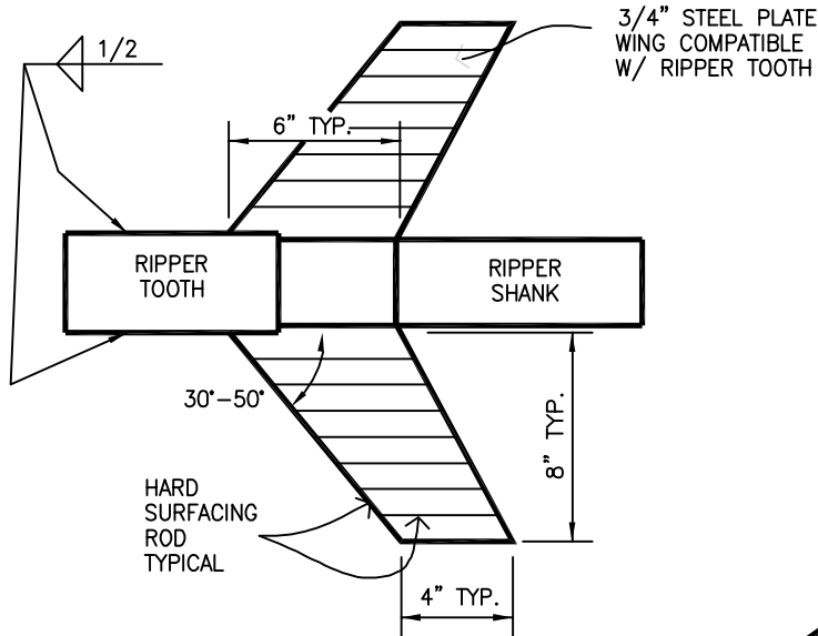
RIPPER — TOP VIEW
