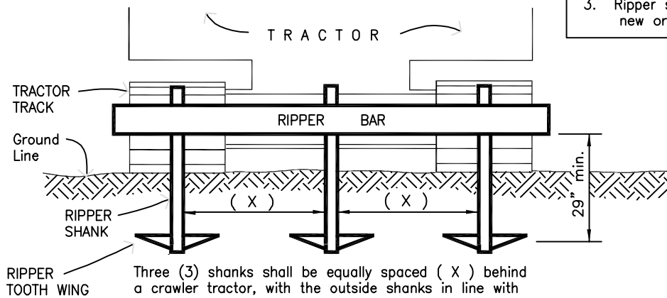
TYPICAL RIPPER POSITIONS
