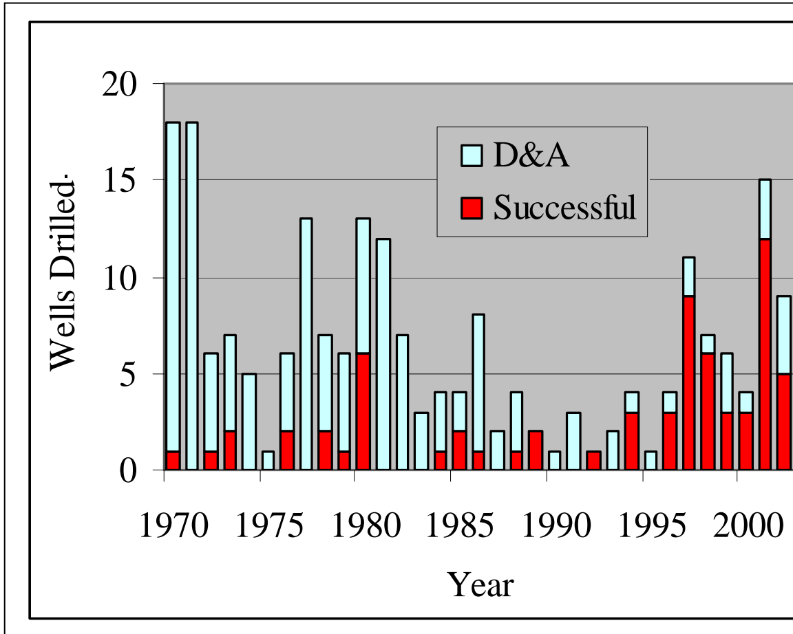
Figure 19. Exploration wells drilled in the Pinedale Field Office area (1970-2002). Note the increased success rate starting in 1996. Data for 2002 are incomplete. Data are from Wyoming Oil and Gas Conservation Commission (2003) and IHS Energy Group (2002).
