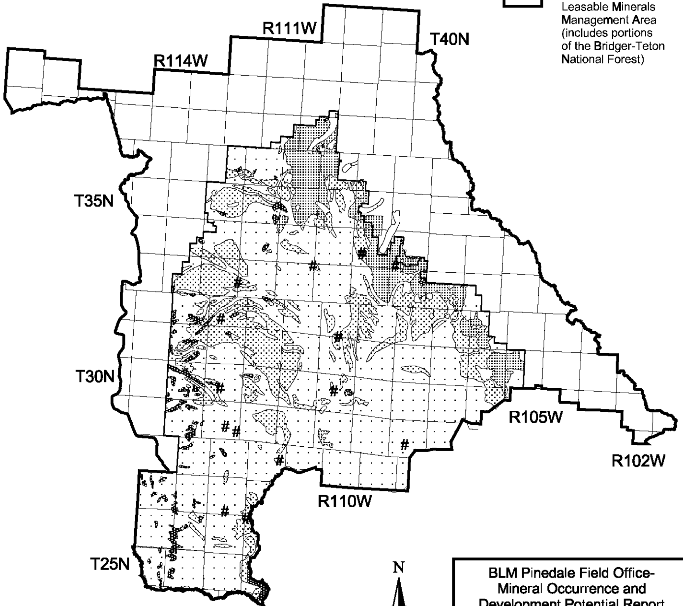
Figure 3-15 Surficial Geology
