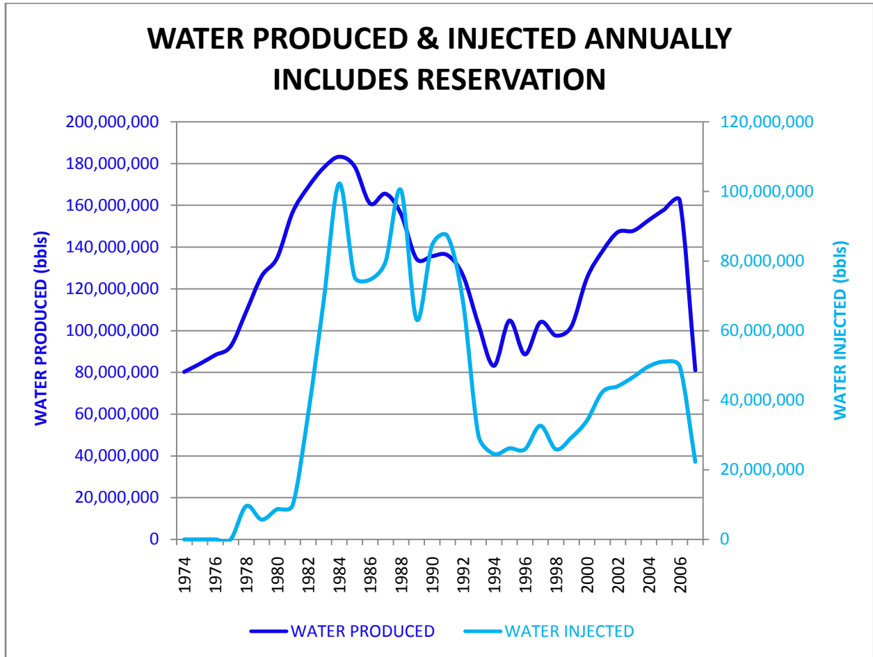
Figure 18. Yearly water injection and water production rates within the Lander Planning Area. Data from IHS Energy Group (2008).
