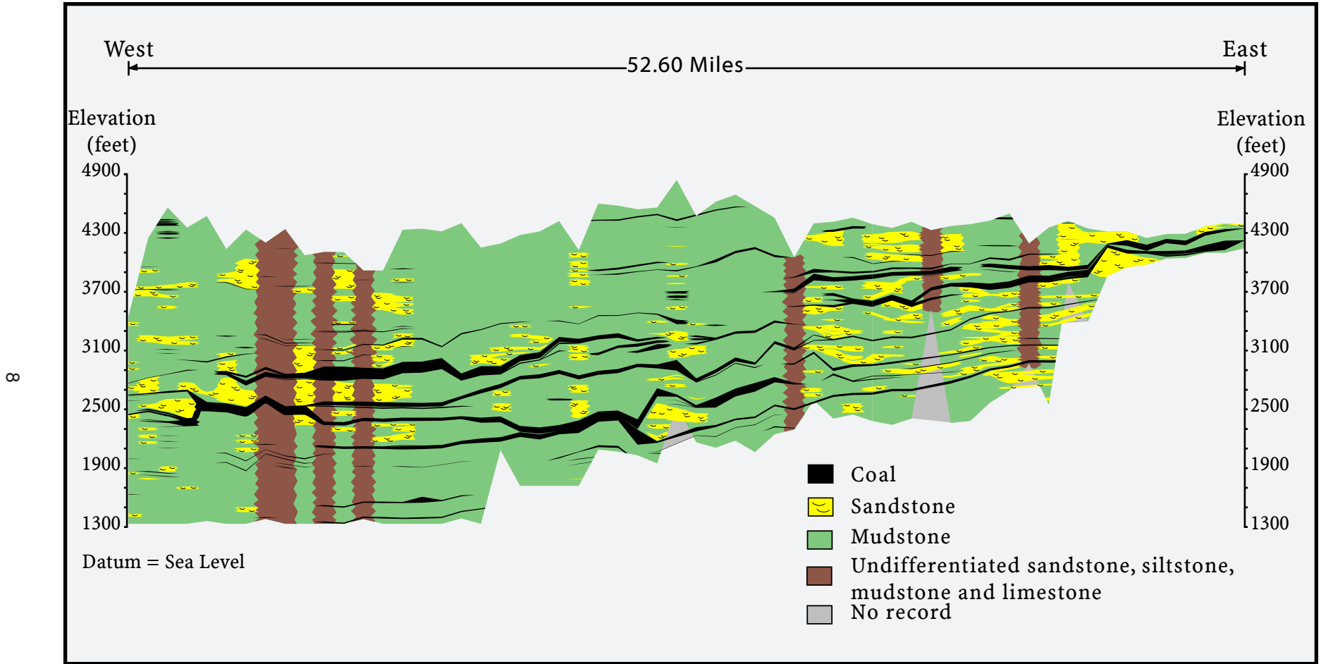
Figure 2. Cross section showing an example of the complex stratigraphic relationship of coal beds in part of the Tongue River Member of the Fort Union Formation. This cross section is in the central part of the Powder River Basin, Wyoming near the city of Gillette. (Modified from Flores and others, 1999).
