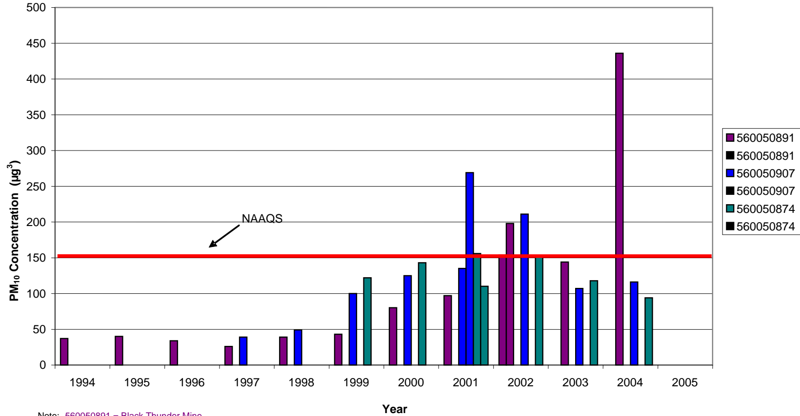
Figure 3-4 PM 10 24-hour Concentrations for Select Black Thunder and North Rochelle Sites
