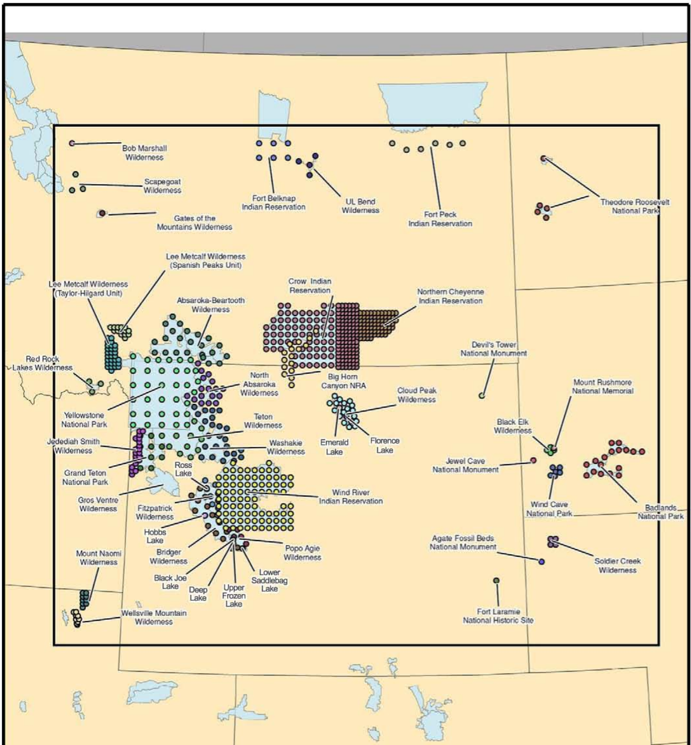
Powder River Basin Coal Review Figure 2-2 Receptor Locations for Sensitive Areas
