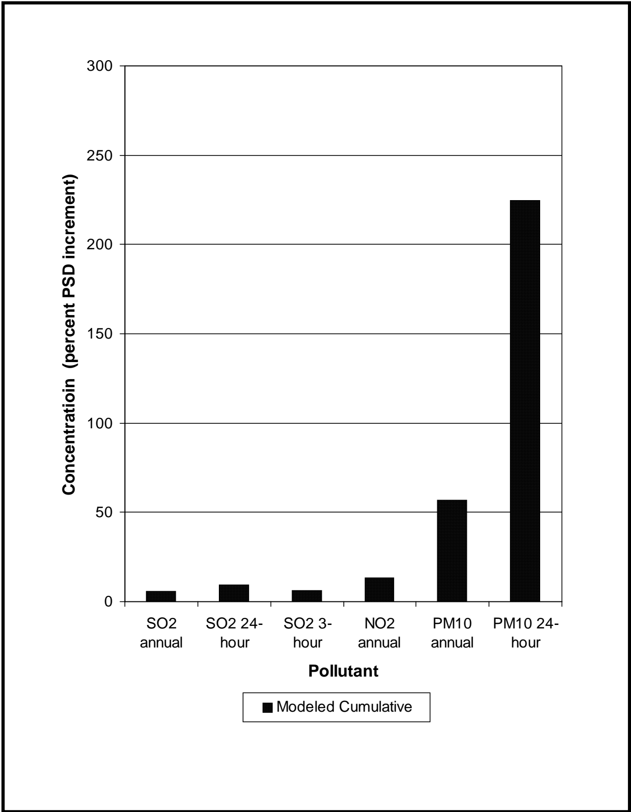
Figure H-2. Comparison of Air Pollutant Concentrations with Prevention of Significant Deterioration Increments.
