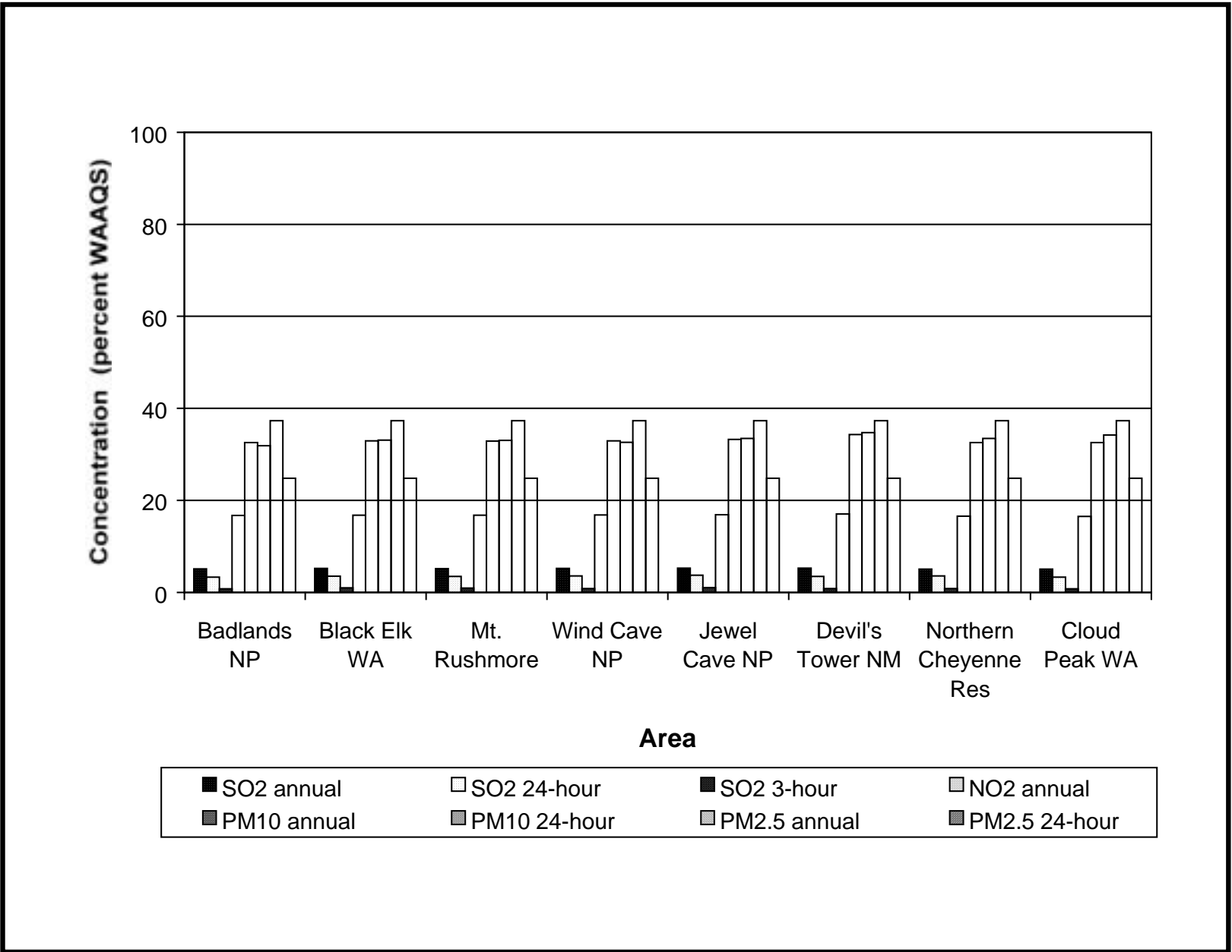
Figure H-3. Comparison of Air Pollutant Concentration with Wyoming Ambient Air Quality Standards.
