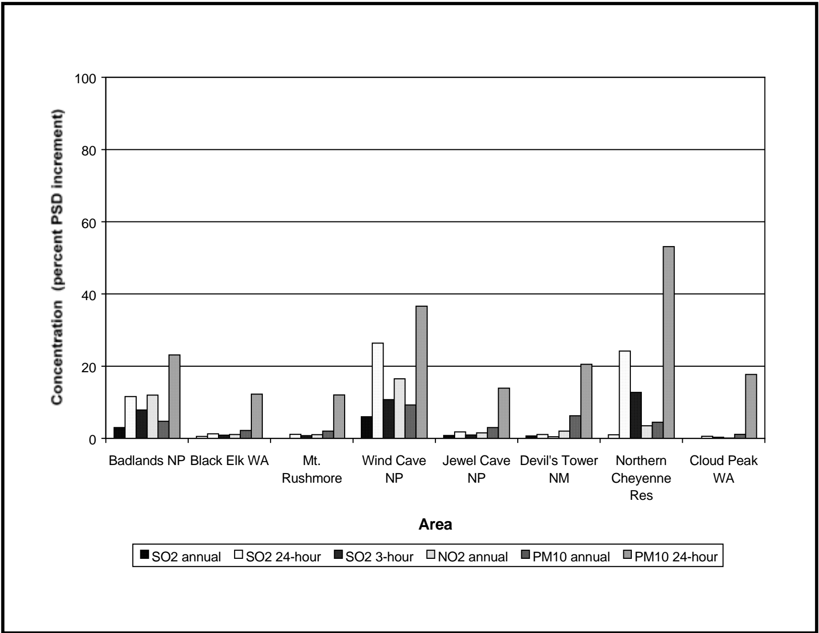
Figure H-4. Comparison of Air Pollutant Concentrations with Prevention of Significant Deterioration Increments.
