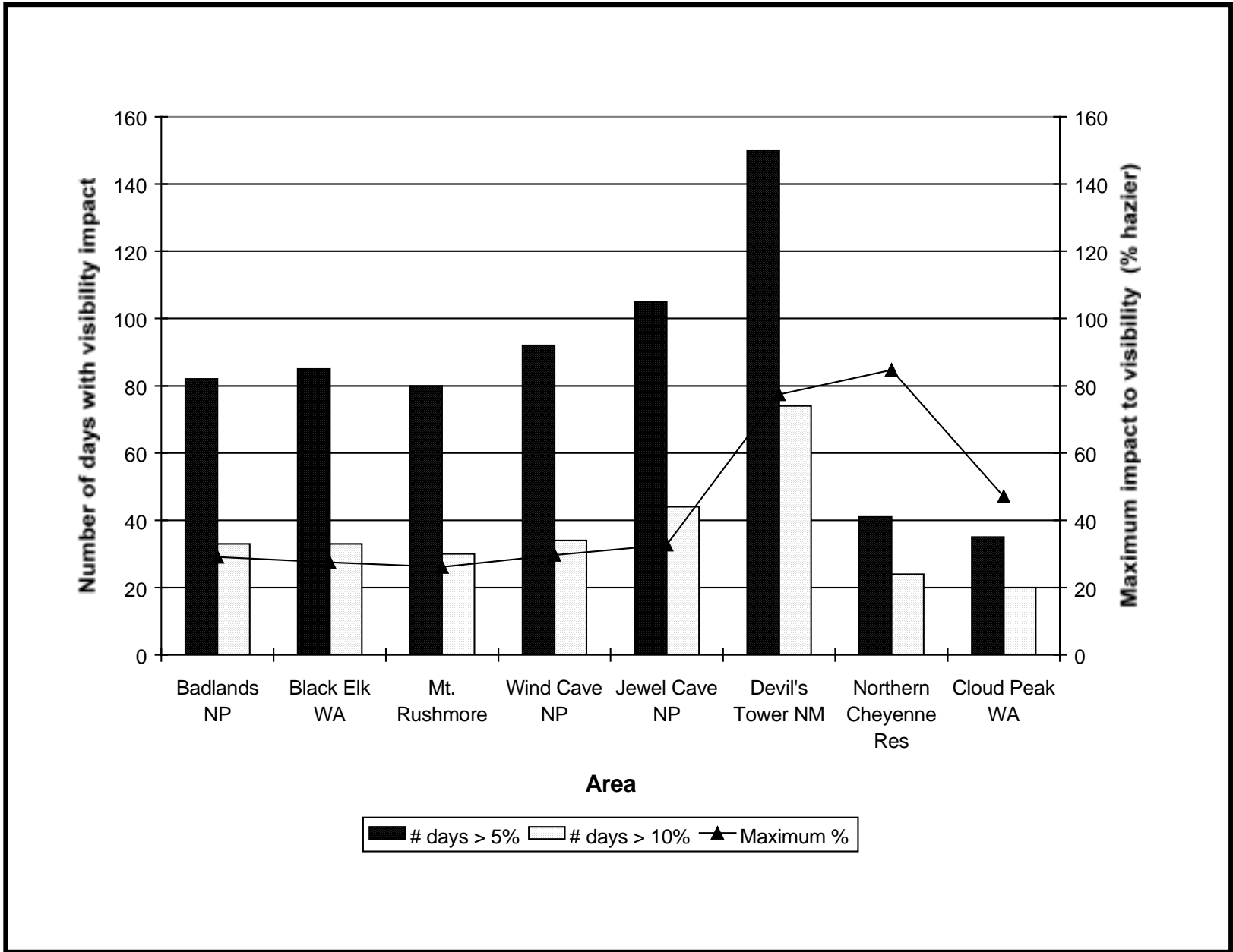
Figure H-6. Worst Case Visibility Impact from DM&E Project.
