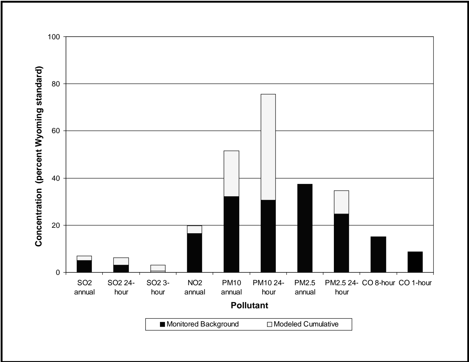
Figure H-1. Comparison of Air Pollutant Concentrations with Wyoming Ambient Air Quality Standards.
