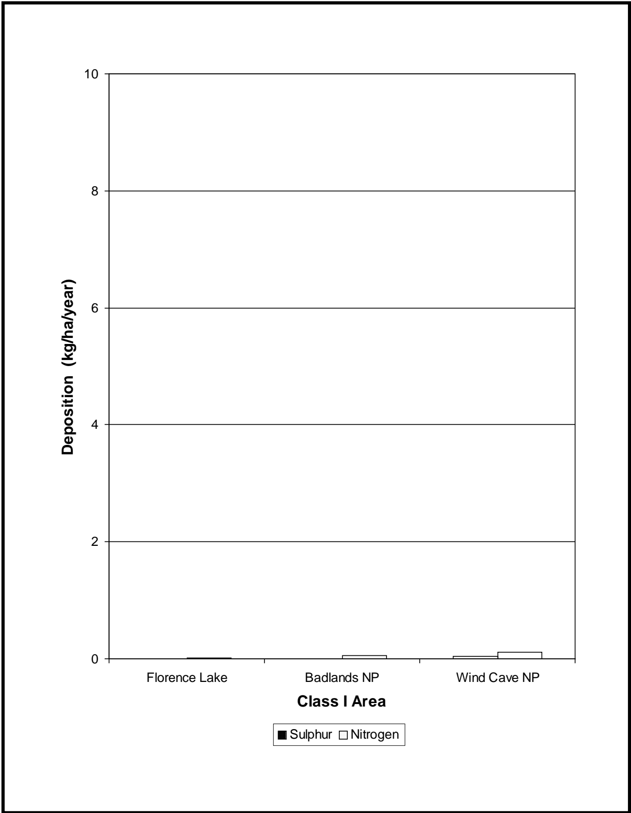
Figure H-5. Acid Deposition.
