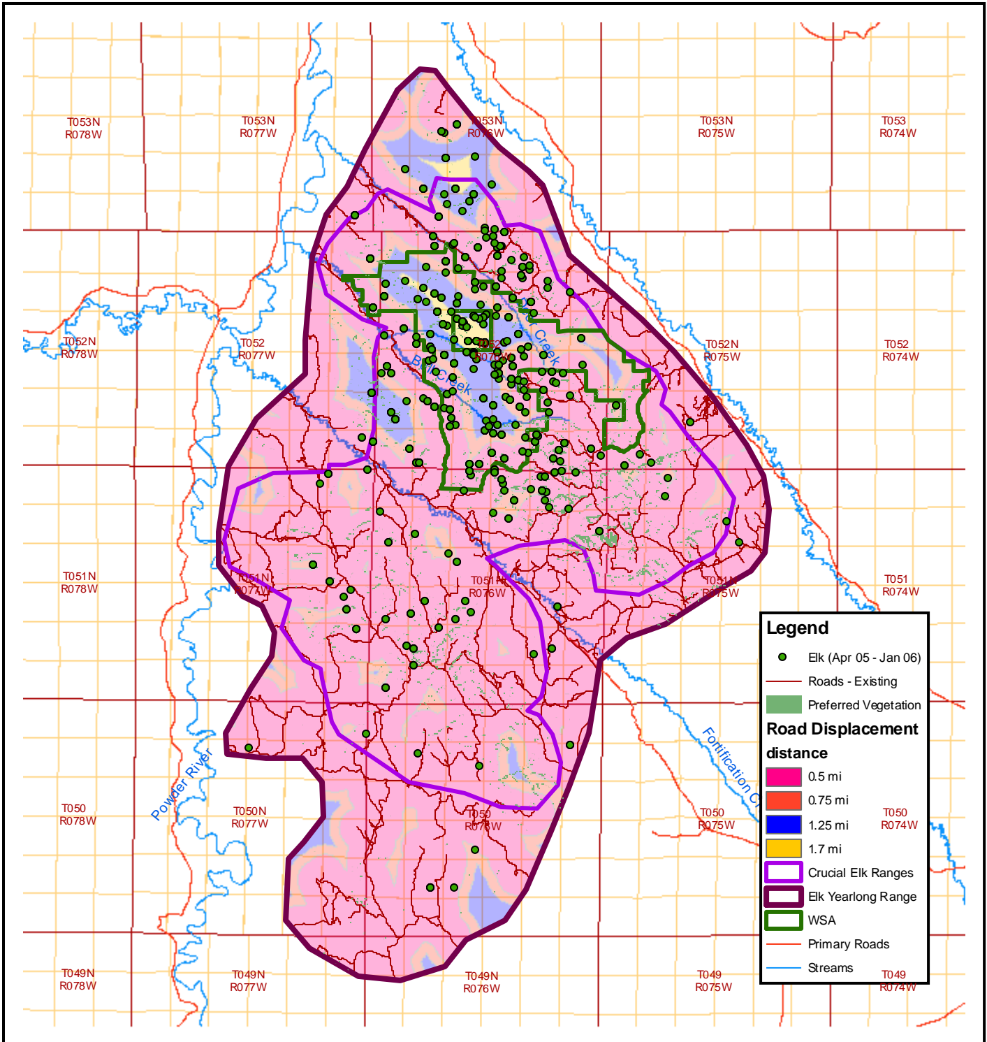
Figure 6. Preferred Vegetation & Elk in Relation to Existing Roads Fortification Creek Area, BLM Buffalo Field Office
