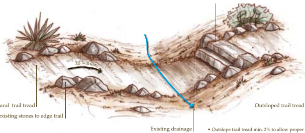
Drainage Crossing On Slope 1/2"=1'-0"
