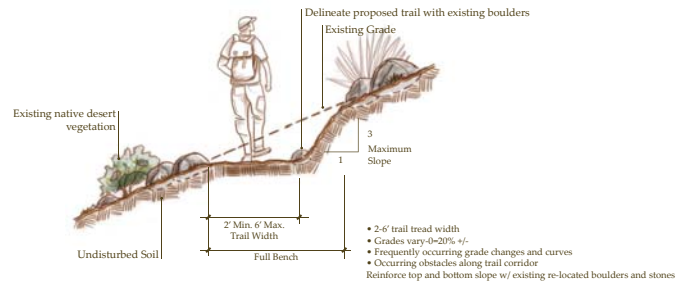
Full Bench Trail on Side Slope-Hiking and Equestrian Wilderness and Non-Wilderness-New 1/2"=1'-0"
