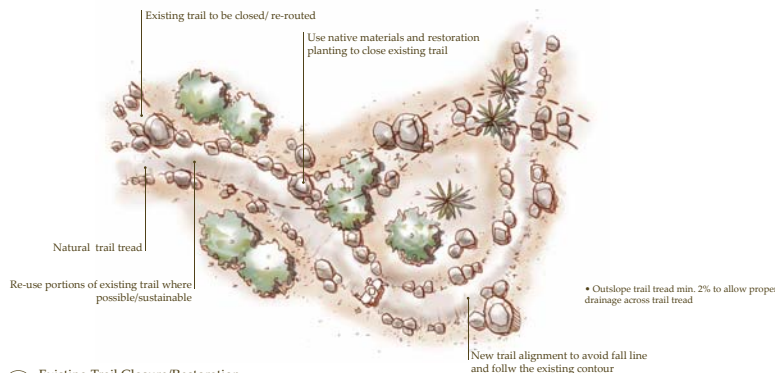
Existing Trail Closure/Restoration 3/8"=1'-0"
