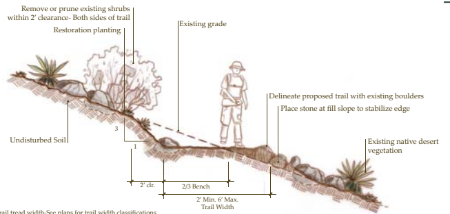
Partial Bench Trail on Side Slope-Hiking and Equestrian Wilderness and Non-Wilderness-New 1/2"=1'-0"
