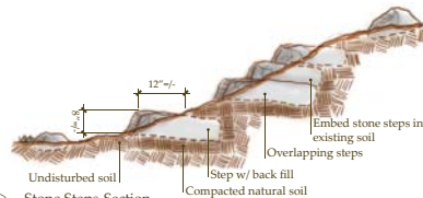
Stone Steps-Section 3/4"=1'-0"
