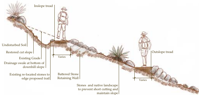
Switchback-Section 1/2"=1'-0"
