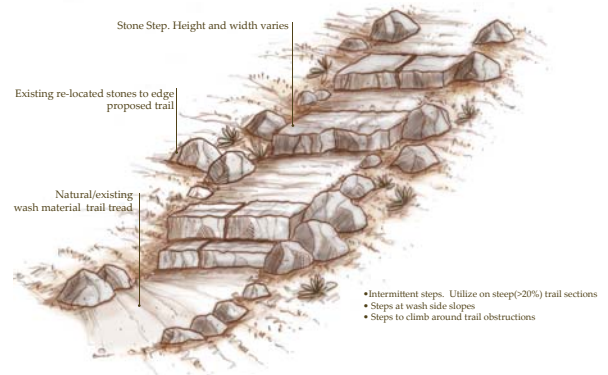
Stone Steps Not to Scale
