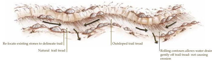
Rolling Contour 1/2"=1'-0"
