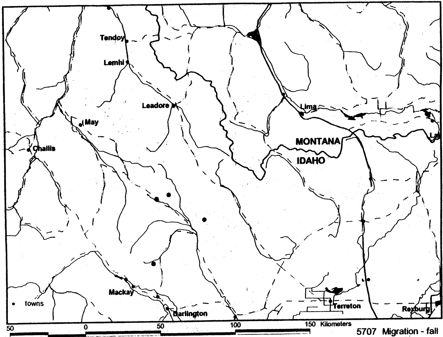
Figure 25. Locations for a subadult female golden eagle (transmitter 5707) in the Intermountain West during fall migration 1996.
