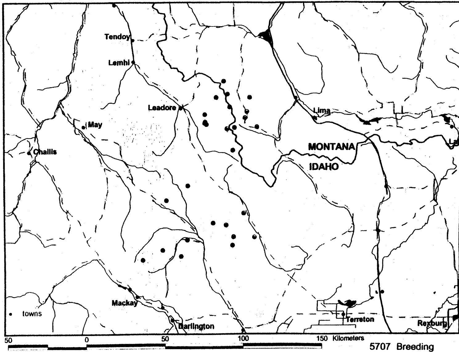
Figure 24. Home range of a subadult female golden eagle (transmitter 5707) in the Intermountain West during breeding season 1996.
