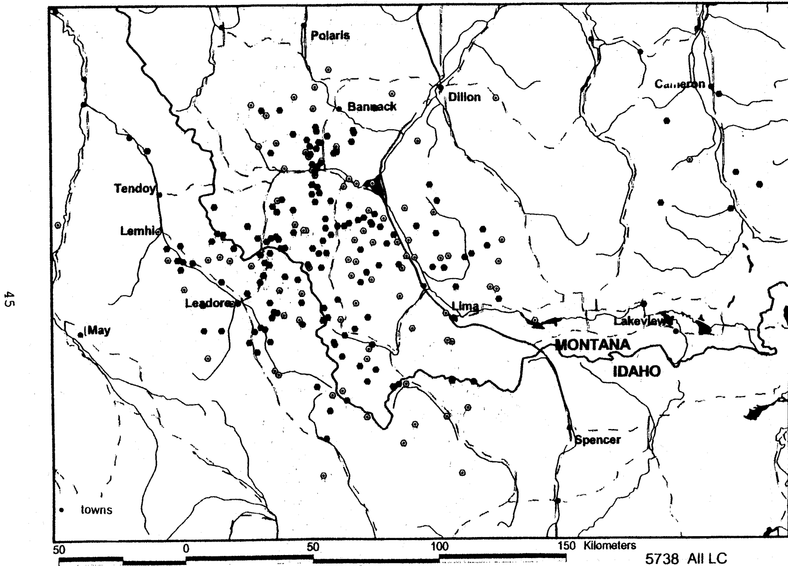
Figure 21. All locations for a subadult male golden eagle (transmitter 5738) in the Intermountain West from 15 January 1996 through 3 January 1997.
