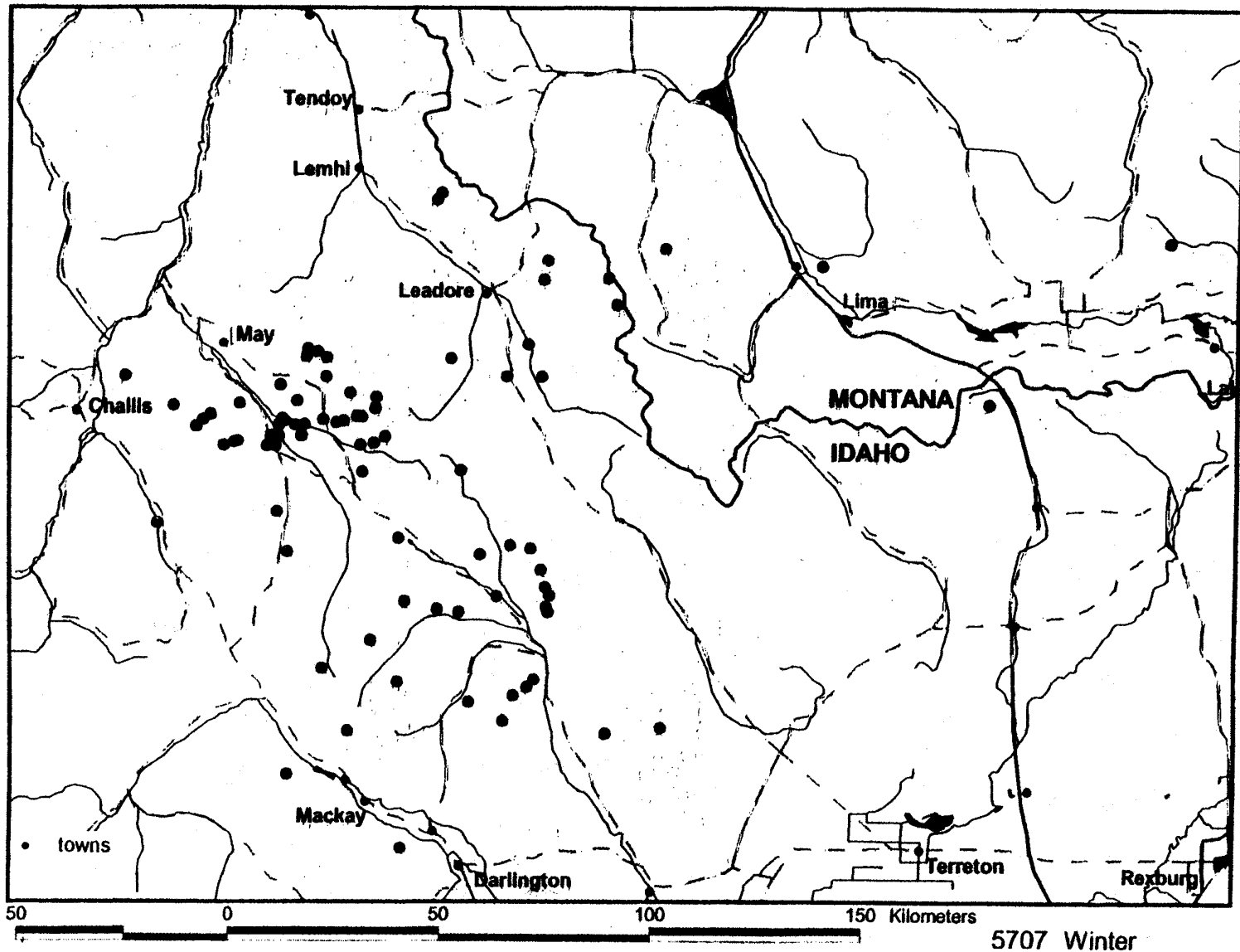
Figure 22. Range of a subadult female golden eagle (transmitter 5707) in the Intermountain West during winter 1995-96.
