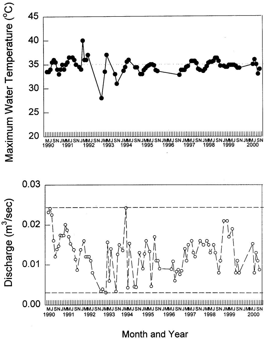
Figure 8. Discharge and maximum water temperatures for Site 1 (Hot Creek). Dashed horizontal lines indicate the maximum and minimum discharges measured at Hot Creek. Dotted horizontal line indicates thermal maximum temperature for P. bruneauensis .
