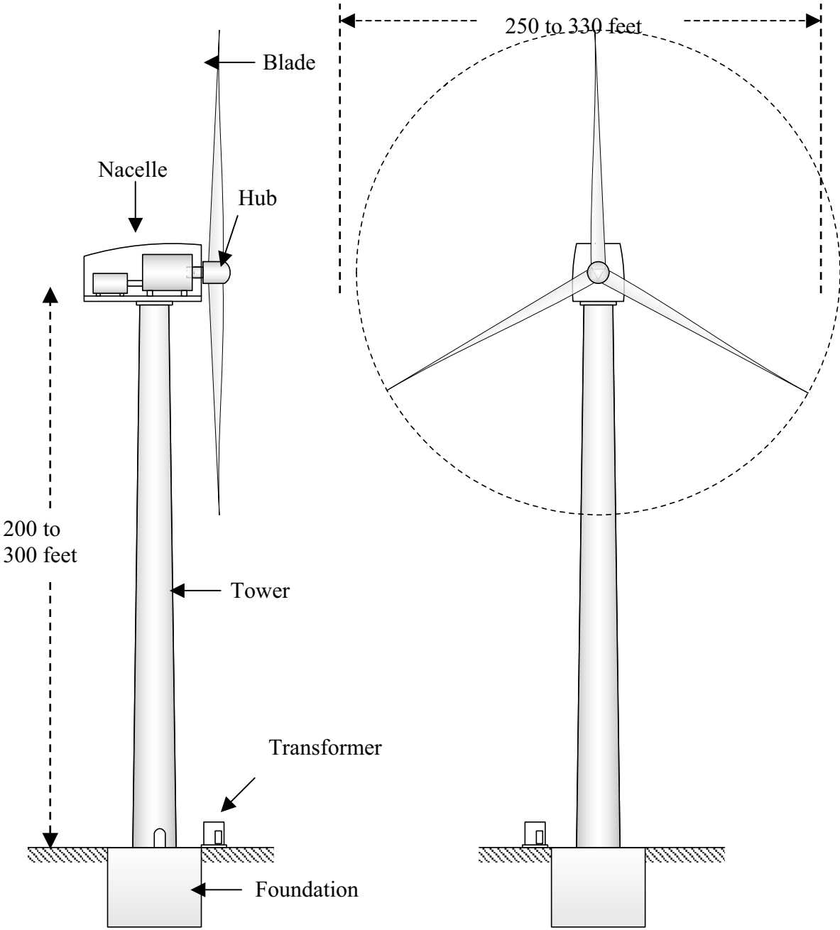
Figure 2-2. General Wind Turbine Components.
