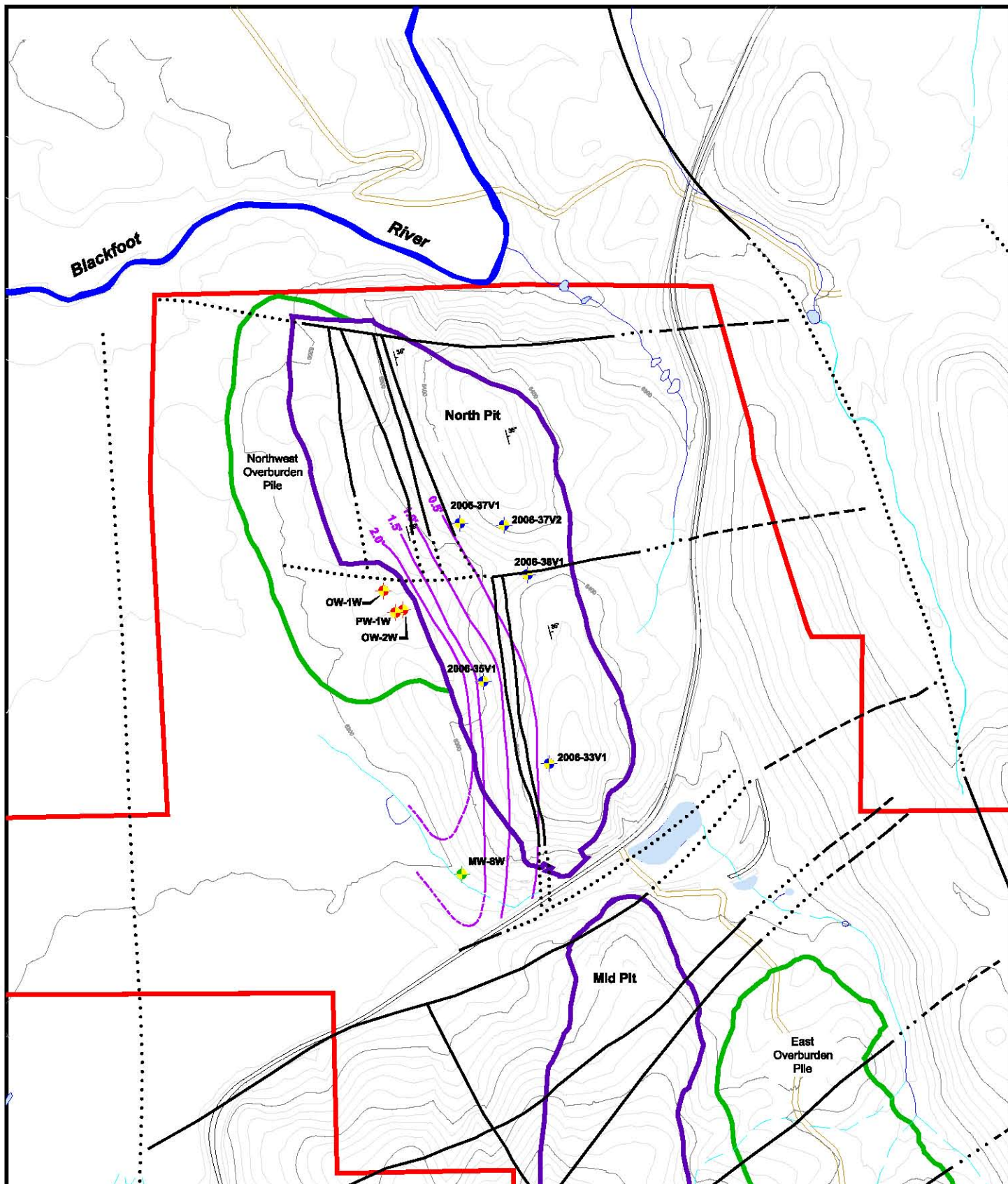
FIGURE 3.3-14 Well Location Map and Maximum Drawdown for Wells Formation Aquifer Test
