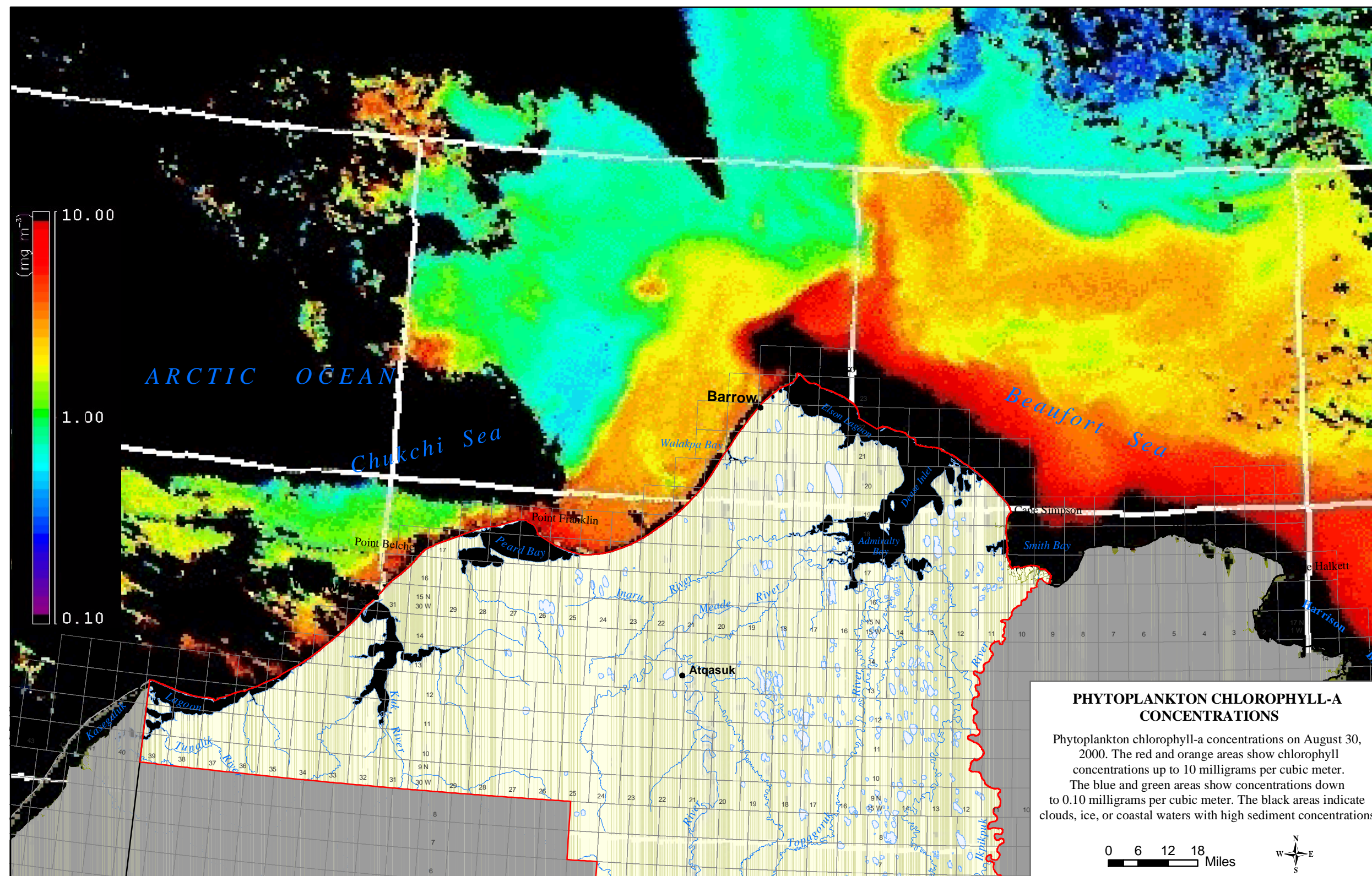
Map 31. Phytoplankton Chlorophyll-A Concentrations Offshore of NPR-A in August 2000
