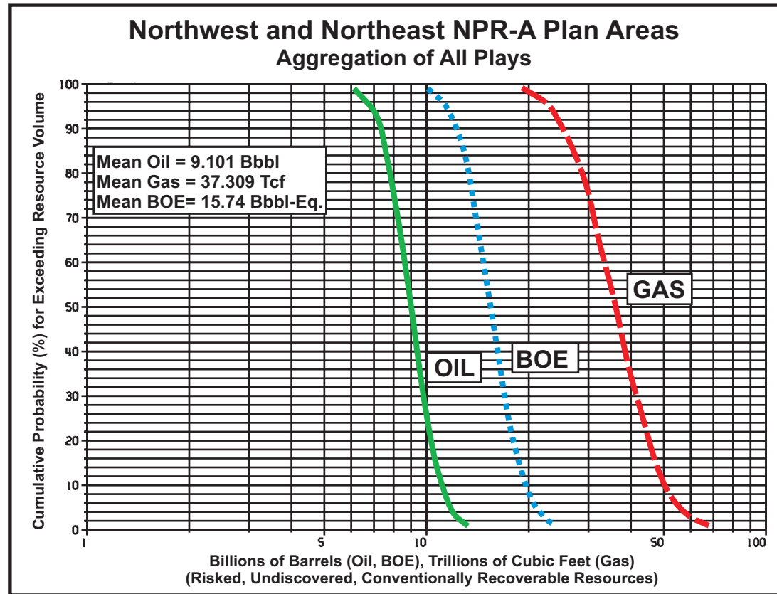
Figure App-02. Cumulative Probability Plot for Conventionally Recoverable Oil and Gas in the Northwest and Northeast NPR-A Planning Areas. Aggregated oil and gas resources are represented as BOE or equivalent barrels of oil (5,620 cubic feet of gas equivalent to 1 barrel of oil). Because of uncertainty, input variables are entered as ranged probability distributions and overall resources are consequently calculated as probability distributions. It is highly probable that small volumes of resources are present but improbable that the maximum possible resource volumes are achieved within the assessment area.
